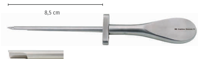
Antrum-Trocar, schnabelförmig, 5,0 x 4,0 mm, AL 8,5 cm, für 4 mm Endoskope Antrum trocar, beaked, 5.0 x 4.0 mm, WL 8.5 cm, for 4 mm endoscopes
